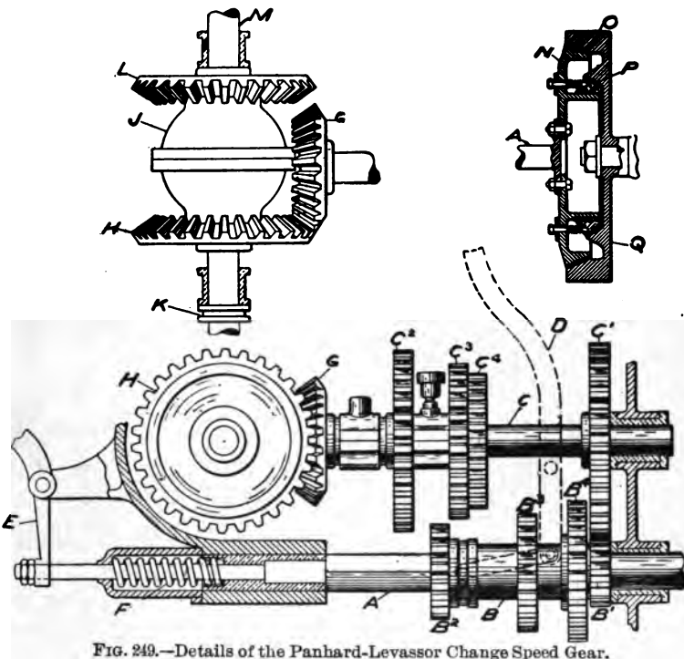
FIG. 249.—Details of the Panhard-Levassor Change Speed Gear.
